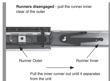
FIG 2b - Removing Runners
