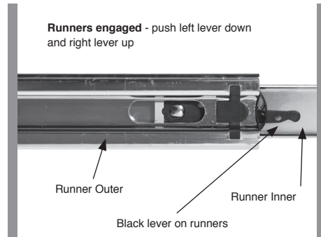
FIG 2a - Removing Runners
